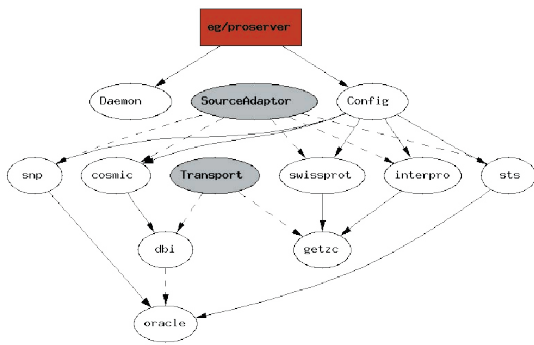
Figure 2: Proserver class diagram. Rectangular box symbol for the main executable script. Ellipsoid shaded boxes for overwritten classes.
