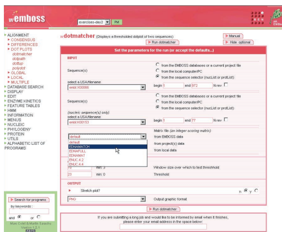
Figure 2. Example of a program page: the dotmatcher.
